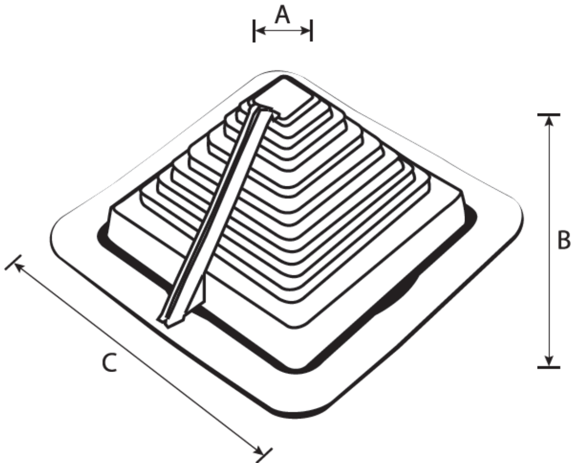
Master Flash® Multi-Flash Square Vent
